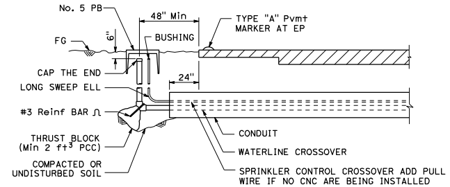
SECTION IRRIGATION CROSSOVER
