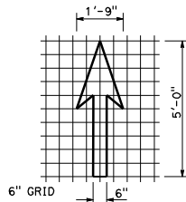
A=7 ft 2 BIKE LANE ARROW
