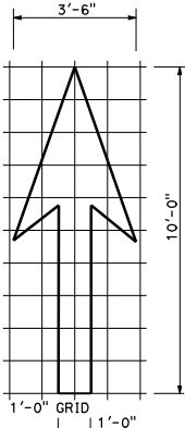
A=14 ft 2 TYPE I 10'-0" ARROW
