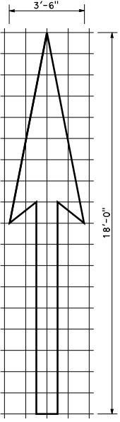
A=25 ft 2 TYPE I 18'-0" ARROW
