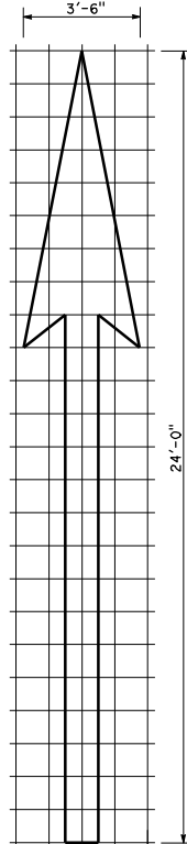
A=31 ft 2 TYPE I 24'-0" ARROW
