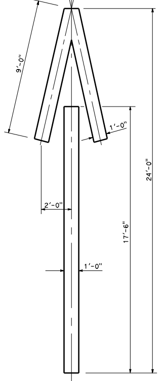
A=33 ft 2 TYPE V ARROW
