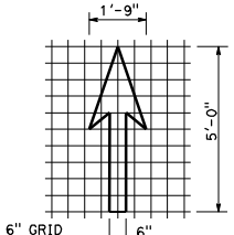
A=7 ft 2 BIKE LANE ARROW
