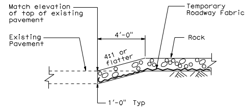
SECTION CONFORM DETAIL
