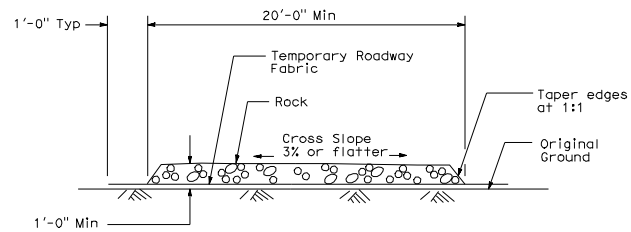
SECTION TEMPORARY CONSTRUCTION ROADWAY
