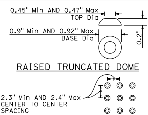
RAISED TRUNCATED DOME RAISED TRUNCATED DOME PATTERN (IN-LINE) DETECTABLE WARNING SURFACE
