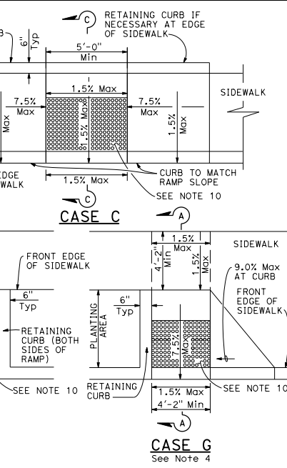
RAISED TRUNCATED DOME RAISED TRUNCATED DOME PATTERN (IN-LINE) DETECTABLE WARNING SURFACE
