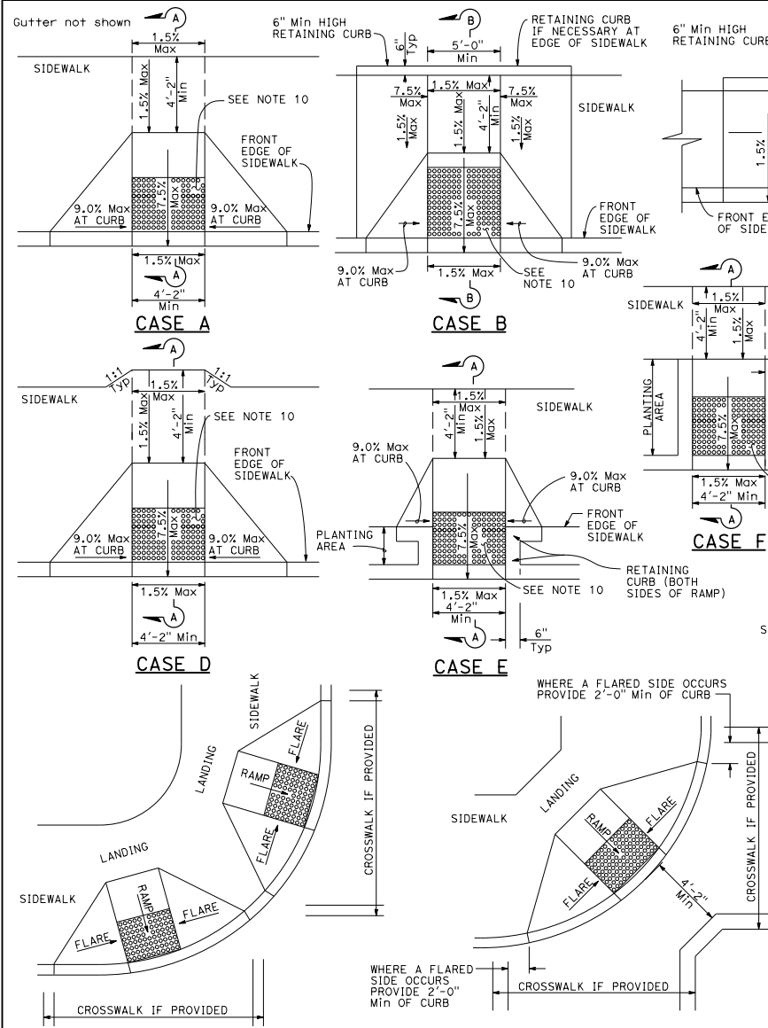
DETAIL A TYPICAL TWO-RAMP CORNER INSTALLATION See Note 1
