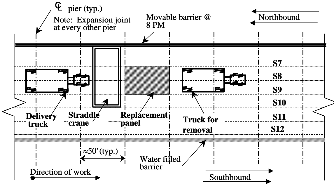
Figure 14. Deck erection and removal procedure for the Inverset TM deck units (N.T.S.). (1 inch = 25.4 mm; 1 foot = 0.3048 meters)
