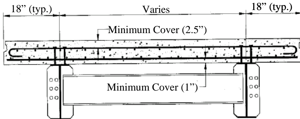
Figure 4. Typical cross section of an Inverset TM deck unit (3). (1 inch = 25.4 mm; 1 foot = 0.3048 meters)
