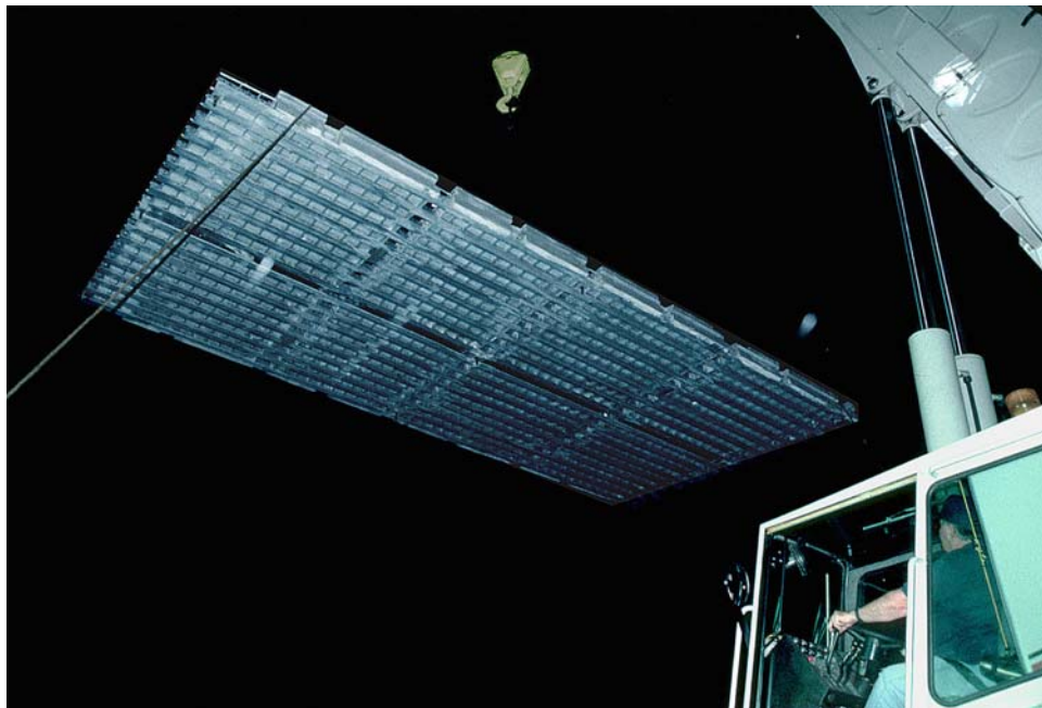
Figure 25. The underside (grid) of a typical Exodermic TM panel during installation.
