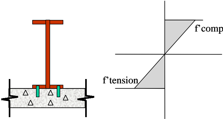
Figure 7. Stress distribution in Inverset TM during casting (3).
