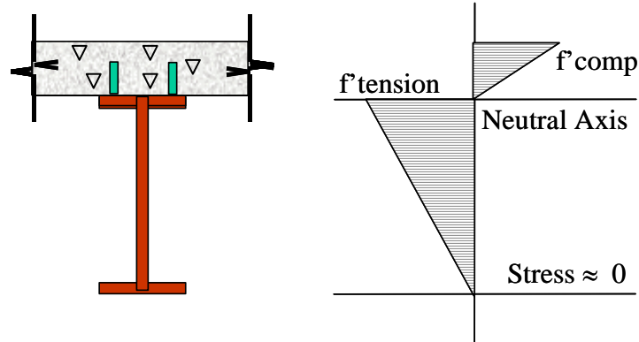
Figure 8. Stress distribution in the composite section (with only dead loads).
