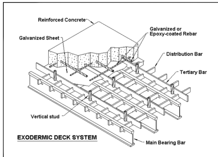
Figure 20. Original Exodermic ™ bridge deck system (6).
