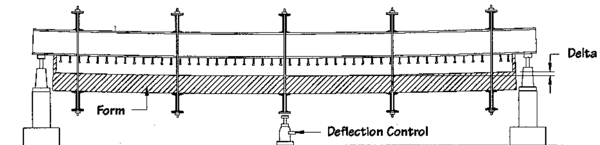
Figure 5. Schematic of the Inverset TM casting process (3).
