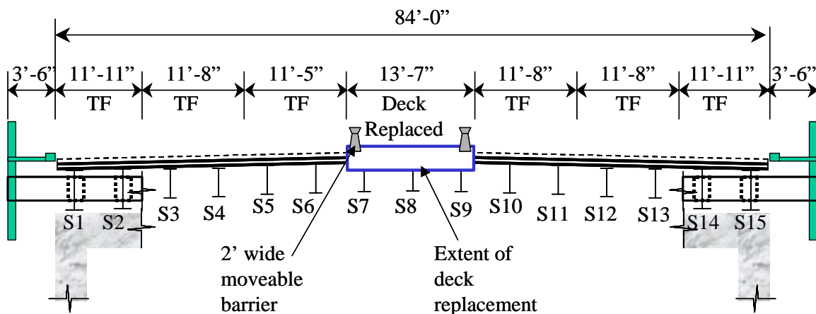
Figure 3. Extent of deck replacement on the west trestle spans (not to scale).
