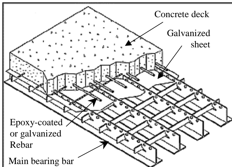
Figure 21. Revised Exodermic TM bridge deck system used in the Tappan Zee Bridge (6).
