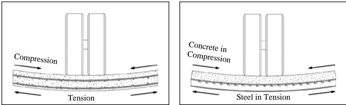
a) Conventional Concrete Deck
