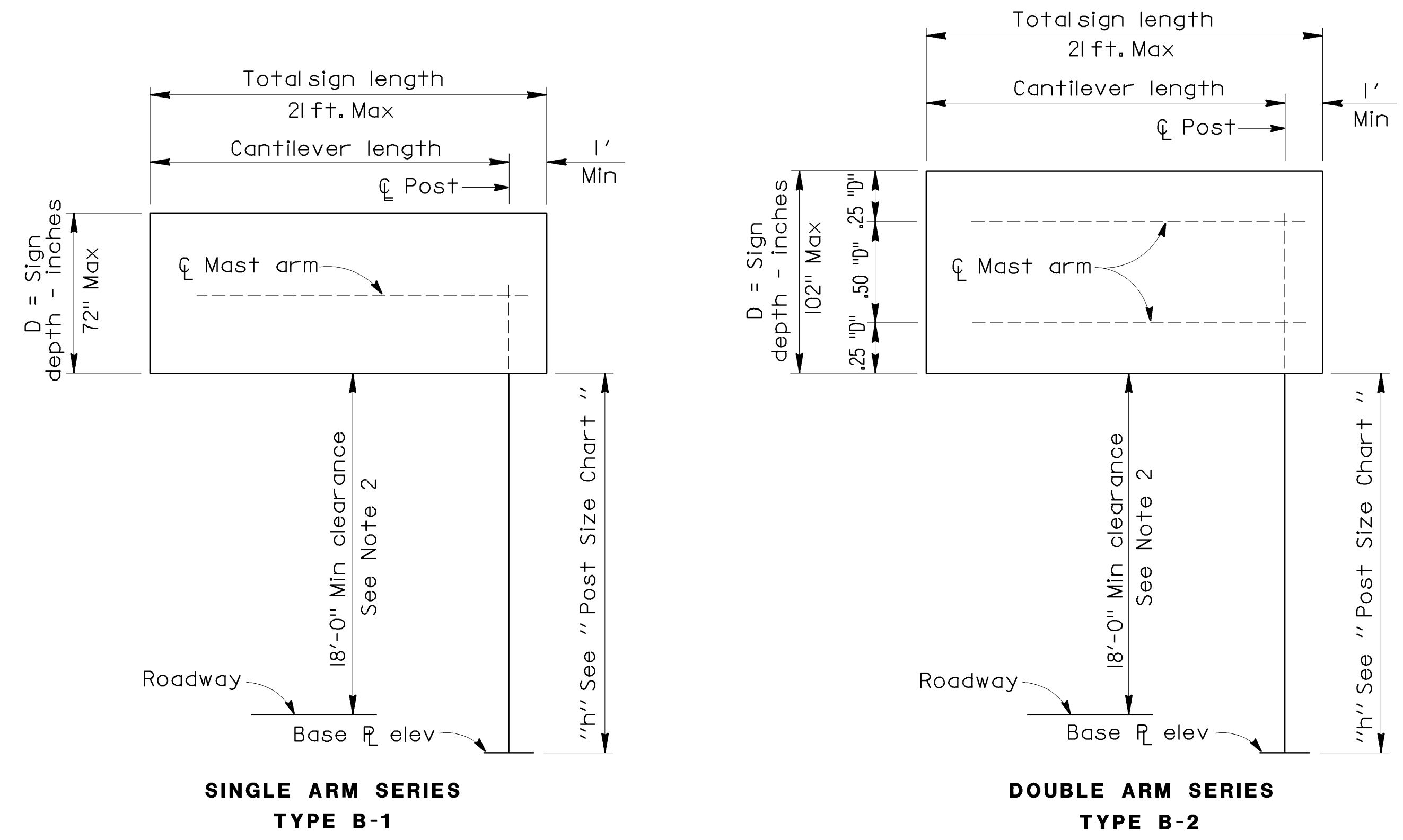
KEY DIMENSION DIAGRAM
