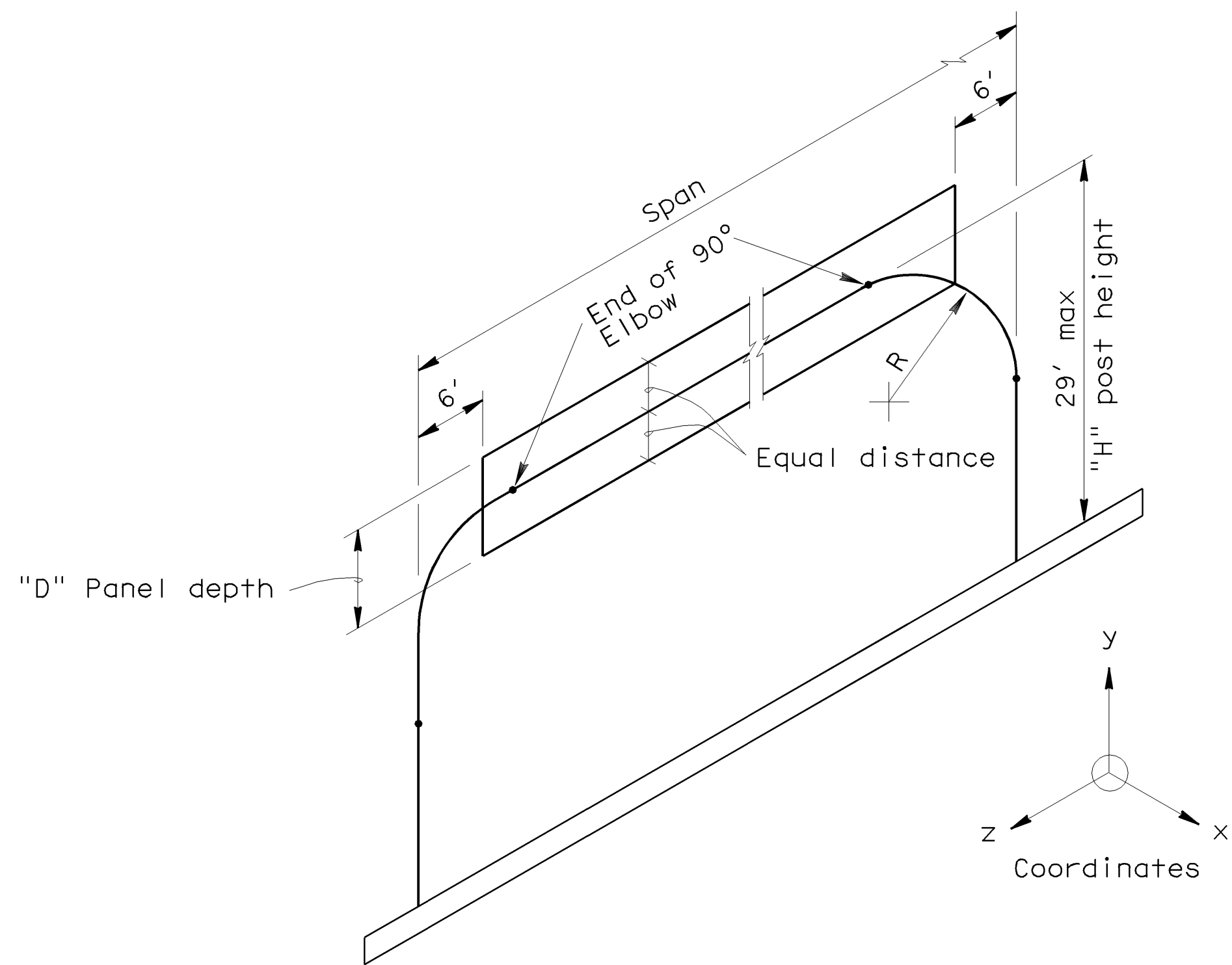
VERTICAL POST 145 FT MAX (Isometric view)
