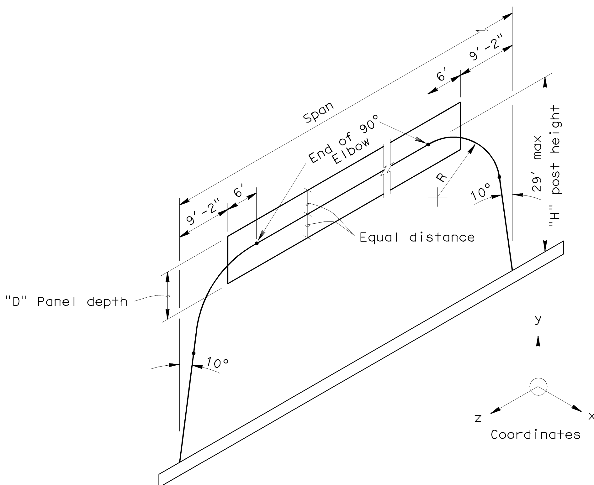
SLANTED POST 145 FT MAX (Isometric view)
