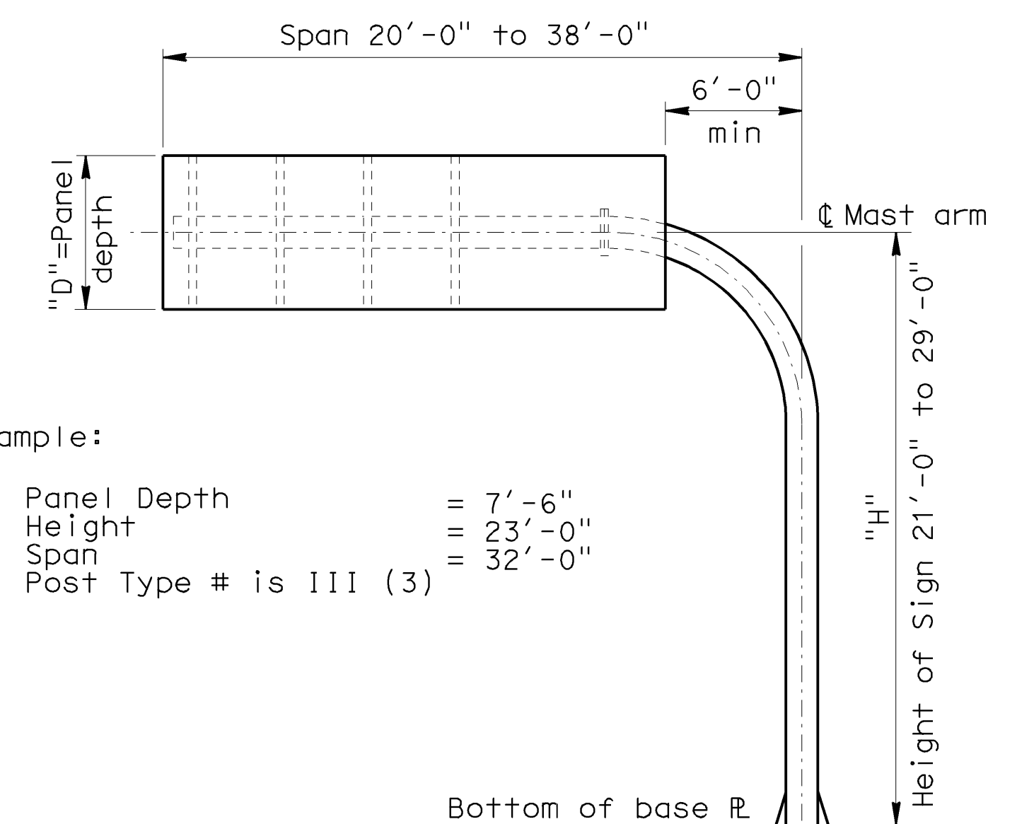
VERTICAL POST CANTILEVER
