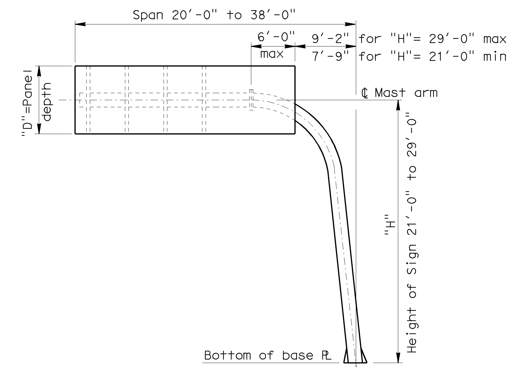
SLANTED POST CANTILEVER
