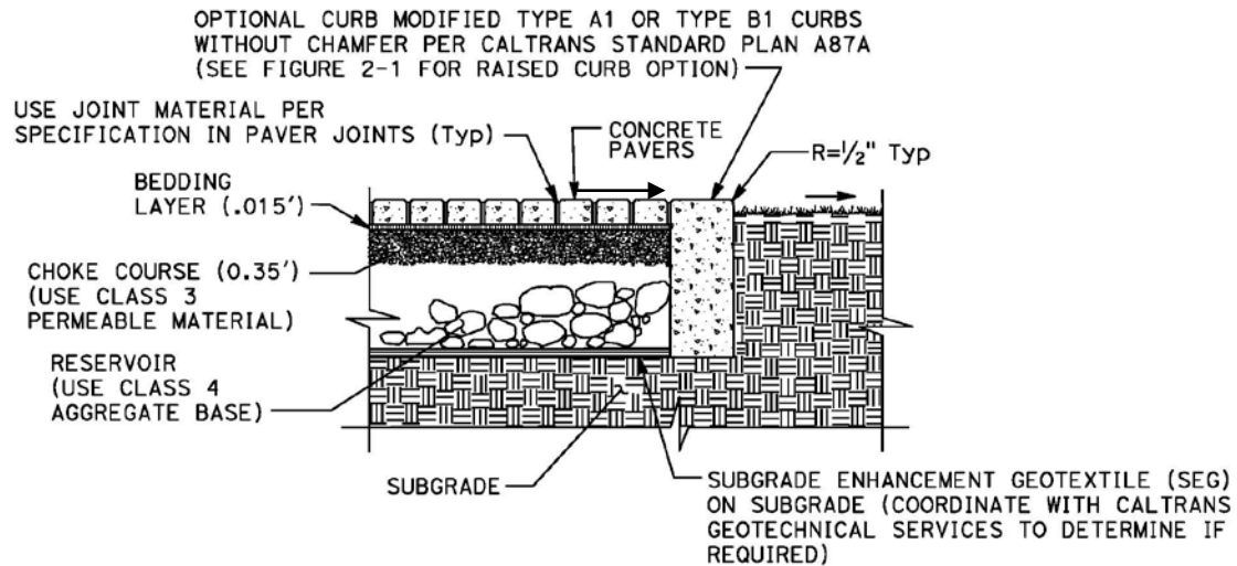
Figure 2-3 - Typical PICP Cross Section
