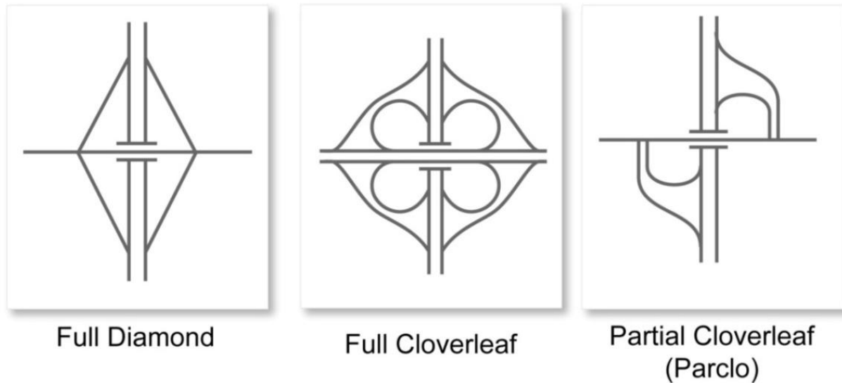
Figure 2: Common interchange designs.
