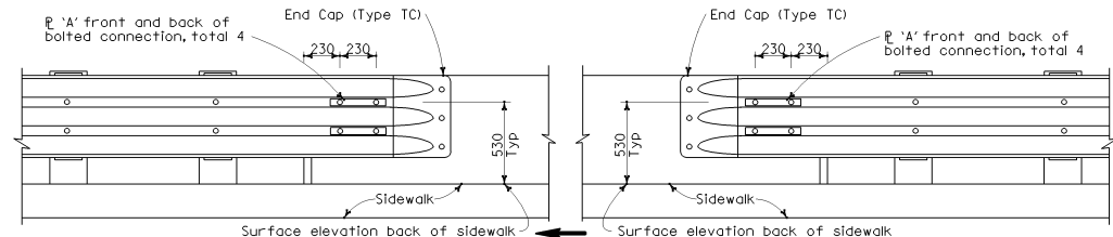
CONNECTION DETAIL HH See Notes 5 CONNECTION DETAIL FF See Notes 4 ELEVATION GUARD RAILING CONNECTION TO BRIDGE RAILING WITH SIDEWALKS
