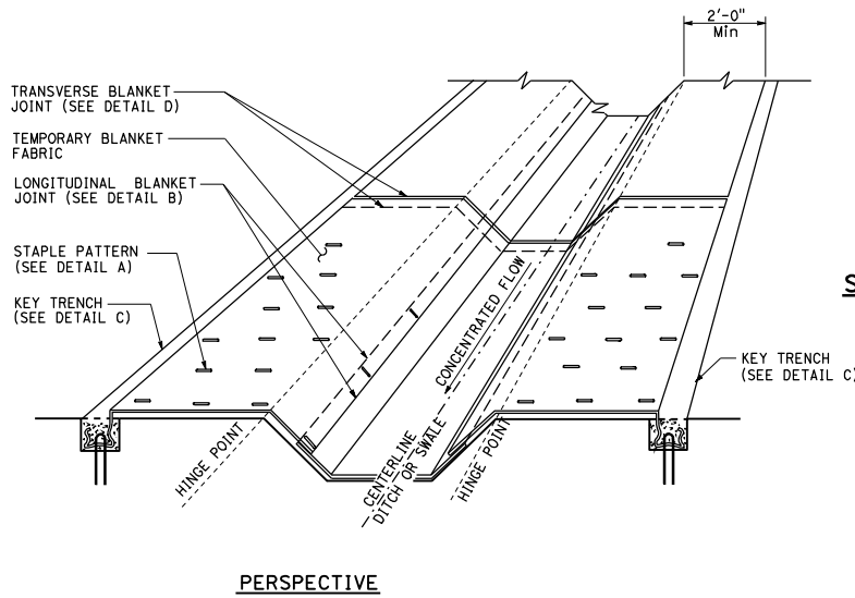
PERSPECTIVE TEMPORARY EROSION CONTROL BLANKET IN TRAPEZOIDAL DITCH OR SWALE
