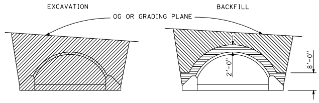
IN TRENCH
