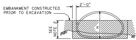
IN EMBANKMENT STRUCTURAL STEEL PLATE PIPE ARCHES AND VEHICULAR UNDERCROSSING
