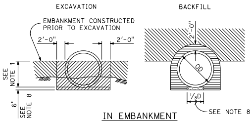
IN EMBANKMENT METAL AND PLASTIC PIPES AND CORRUGATED METAL PIPE ARCHES 84" or Smaller
