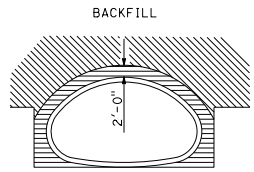
IN EMBANKMENT STRUCTURAL STEEL PLATE PIPE ARCHES AND VEHICULAR UNDERCROSSING
