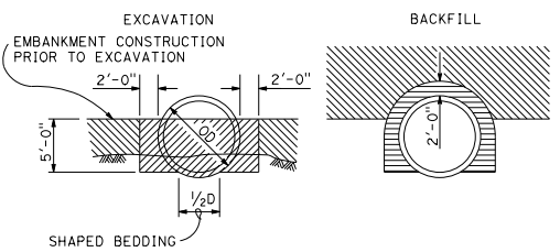
IN EMBANKMENT PIPES Larger than 84"
