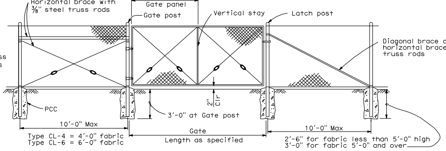
CHAIN LINK GATE INSTALLATION
