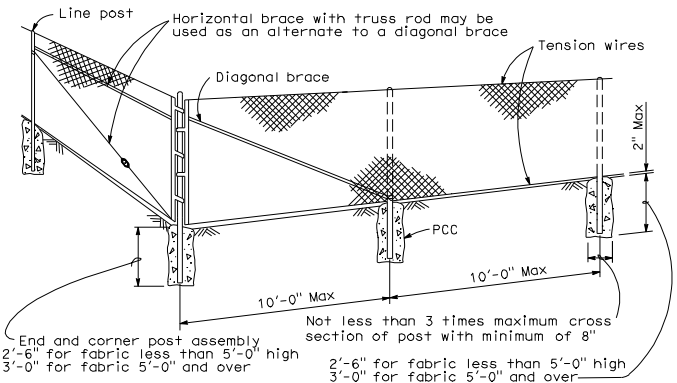
CORNER POST
