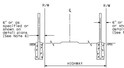
OTHER HIGHWAYS FREEWAYS FENCE LOCATION
