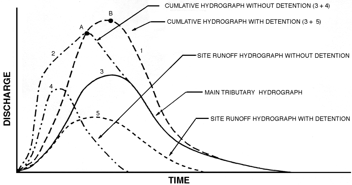
Figure 892.3 Example of Cumulative Hydrograph With and Without Detention
