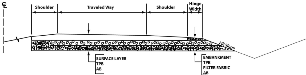
Figure 651.2A Typical Section with Treated Permeable Base Drainage Layer
