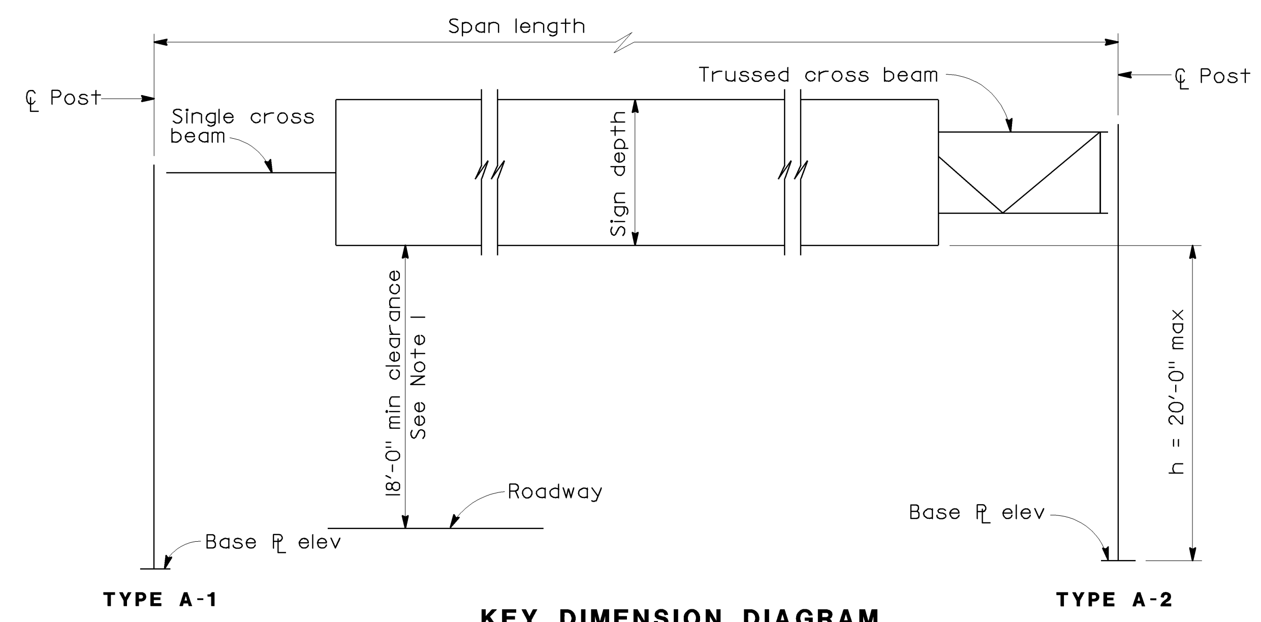
KEY DIMENSION DIAGRAM
