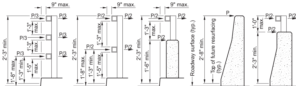
(To be used where there is no curb or curb project 9" or less from traffic face of railing.)
