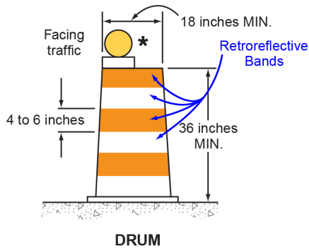
Figure 6F-7. Channelizing Devices
