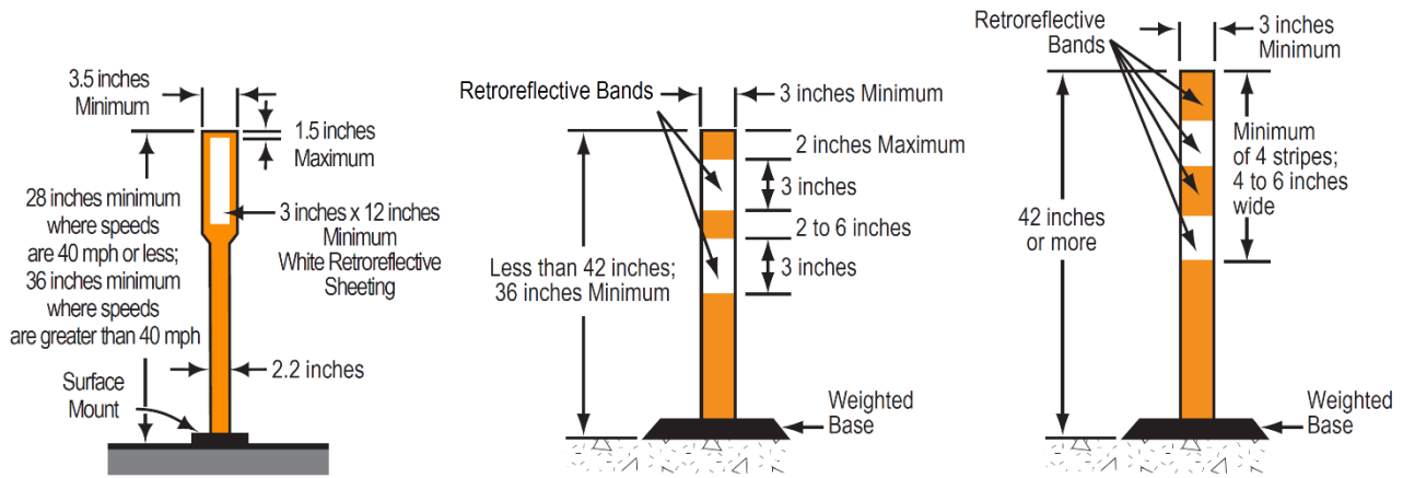
Figure 6F-102 (CA). Tubular Markers
