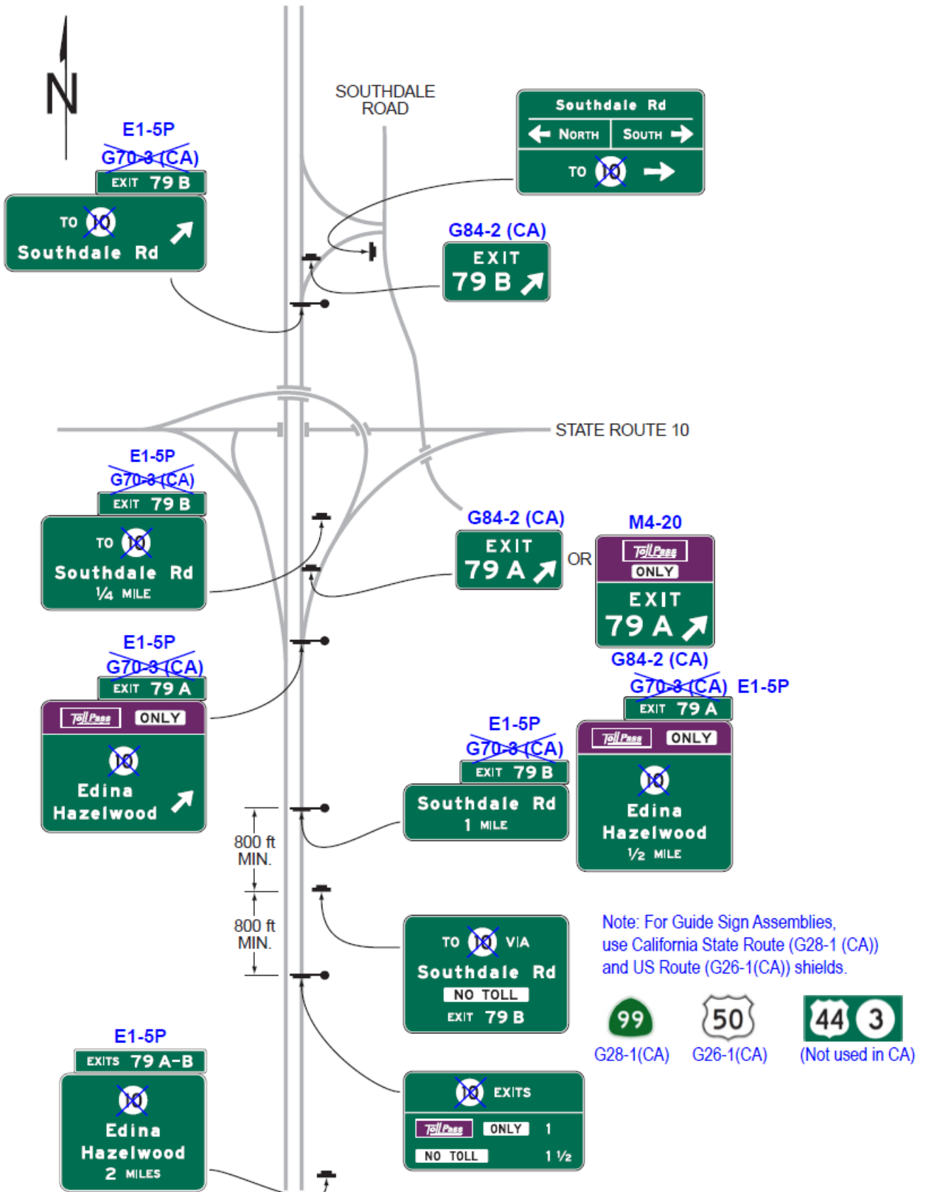
Figure 2F-7. Examples of Guide Signs for Alternative Toll and Non-Toll Ramp Connections to a Non-Toll Highway
