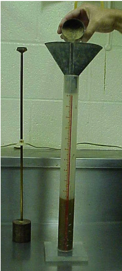
Manually Operated Sand Equivalent Shaker (Idaho Shaker)
